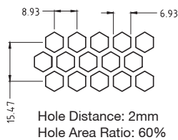
VENTED HOLES
